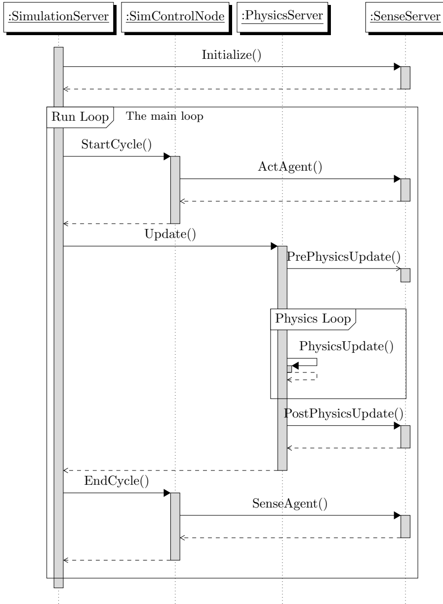
Figure 1: UML sequence diagram demo. The used style-file is pgf-umlsd.sty , you may get it at http://code.google.com/p/pgf-umlsd/
