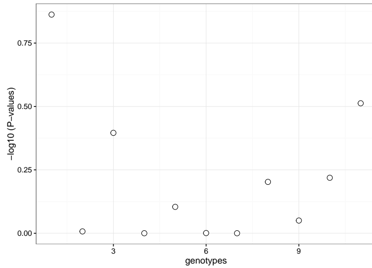
Figure 5: Manhattan plot
