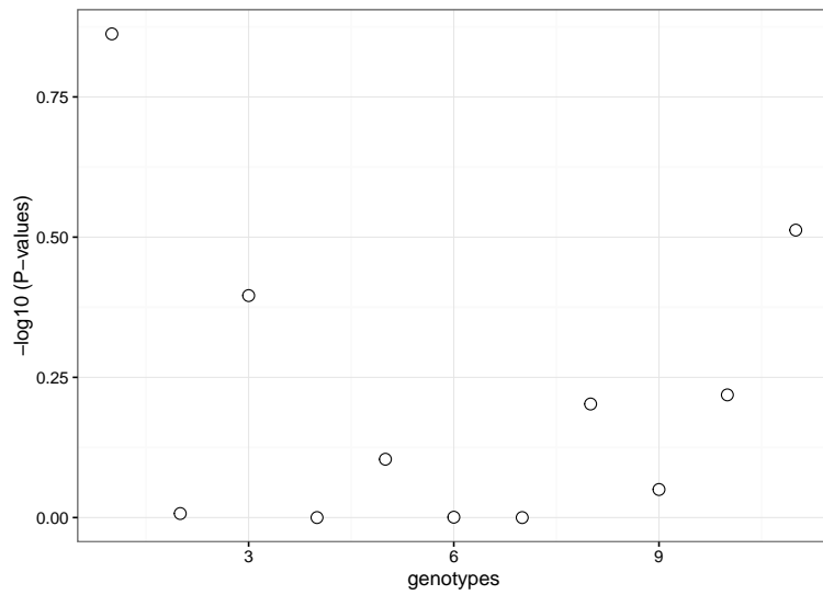
Figure 7: Manhattan plot
