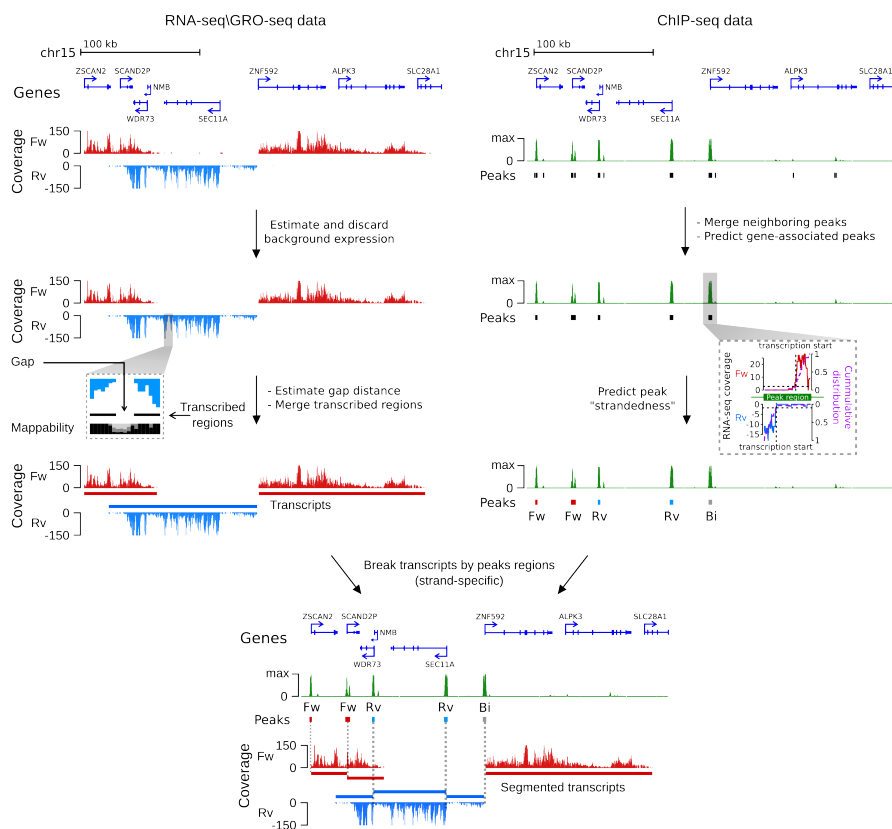
Figure 1: transcriptR workflow
