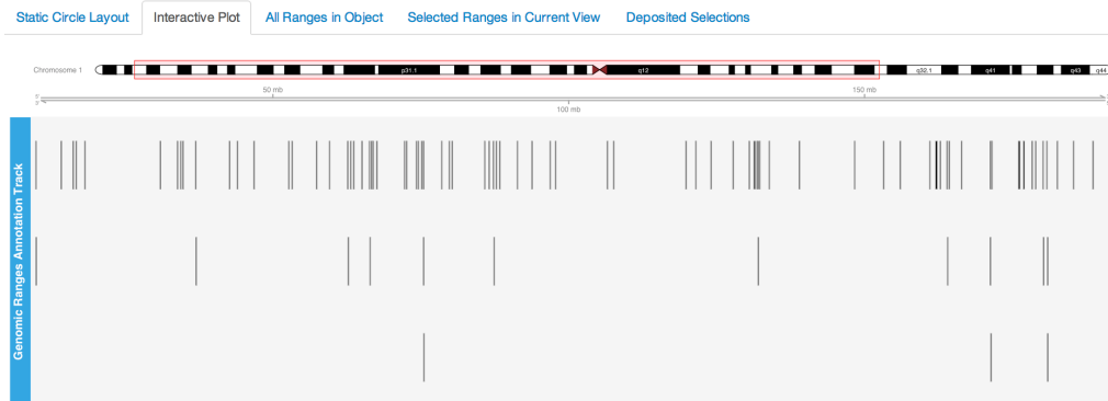
Figure 6: Interactive Plot
